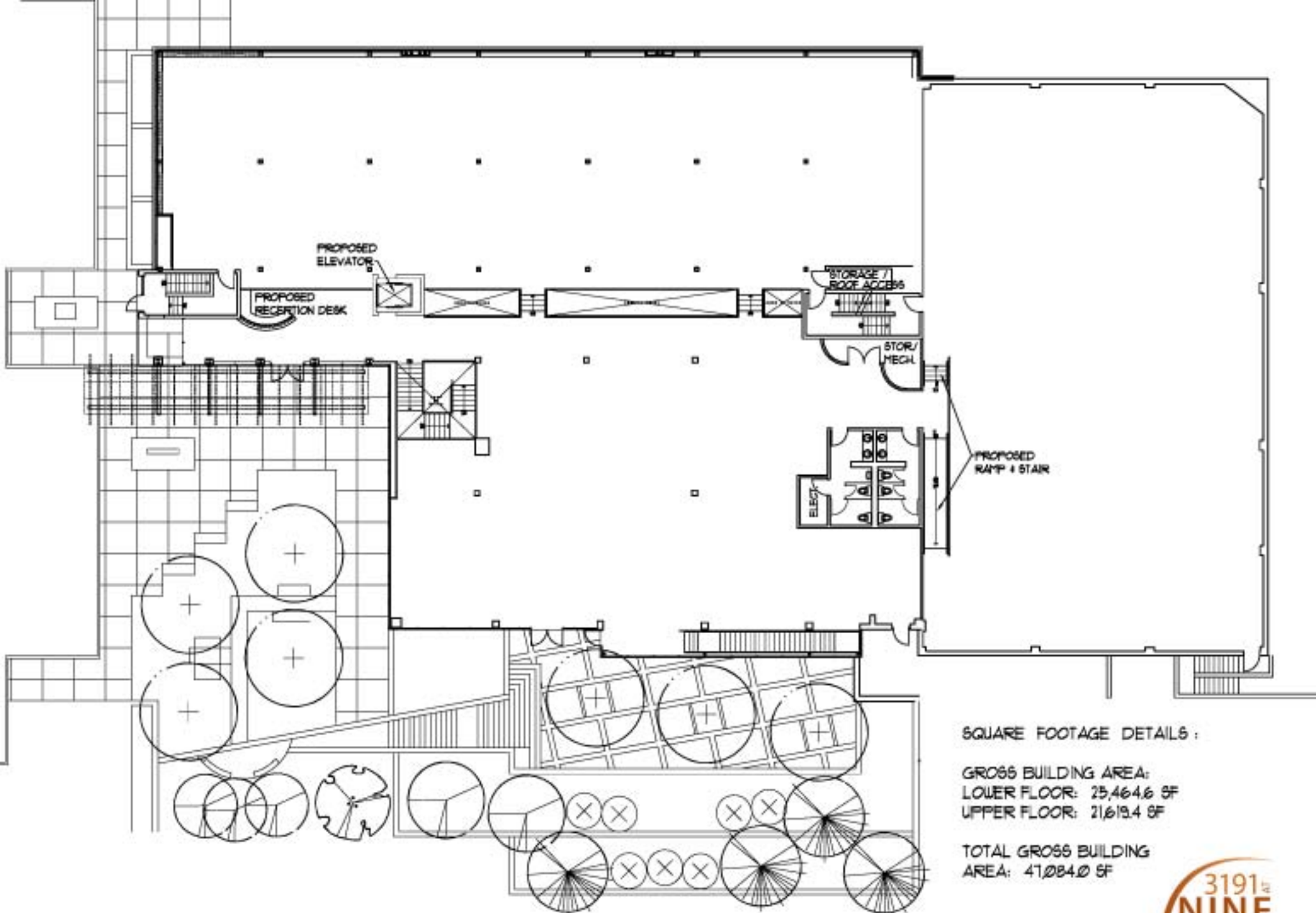
3191 VAUGHN WAY - UPPER LEVEL FLOOR PLAN
